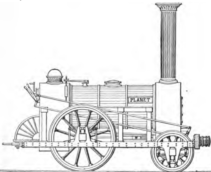
Fig. 20.—“Planet,” No. 9, Liverpool and Manchester Railway, 1830.
